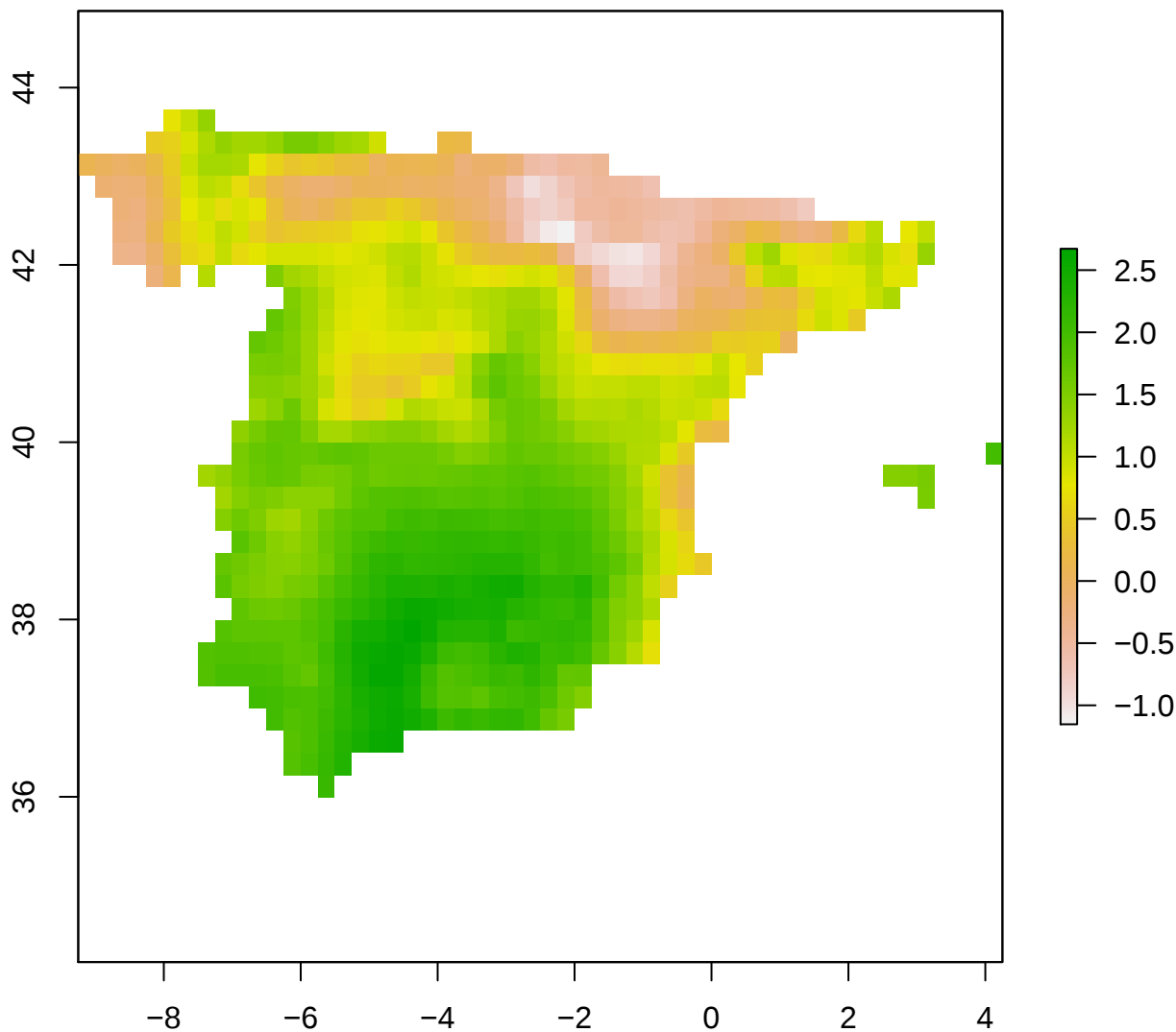
spi12_month - Spain 2010-12-01
