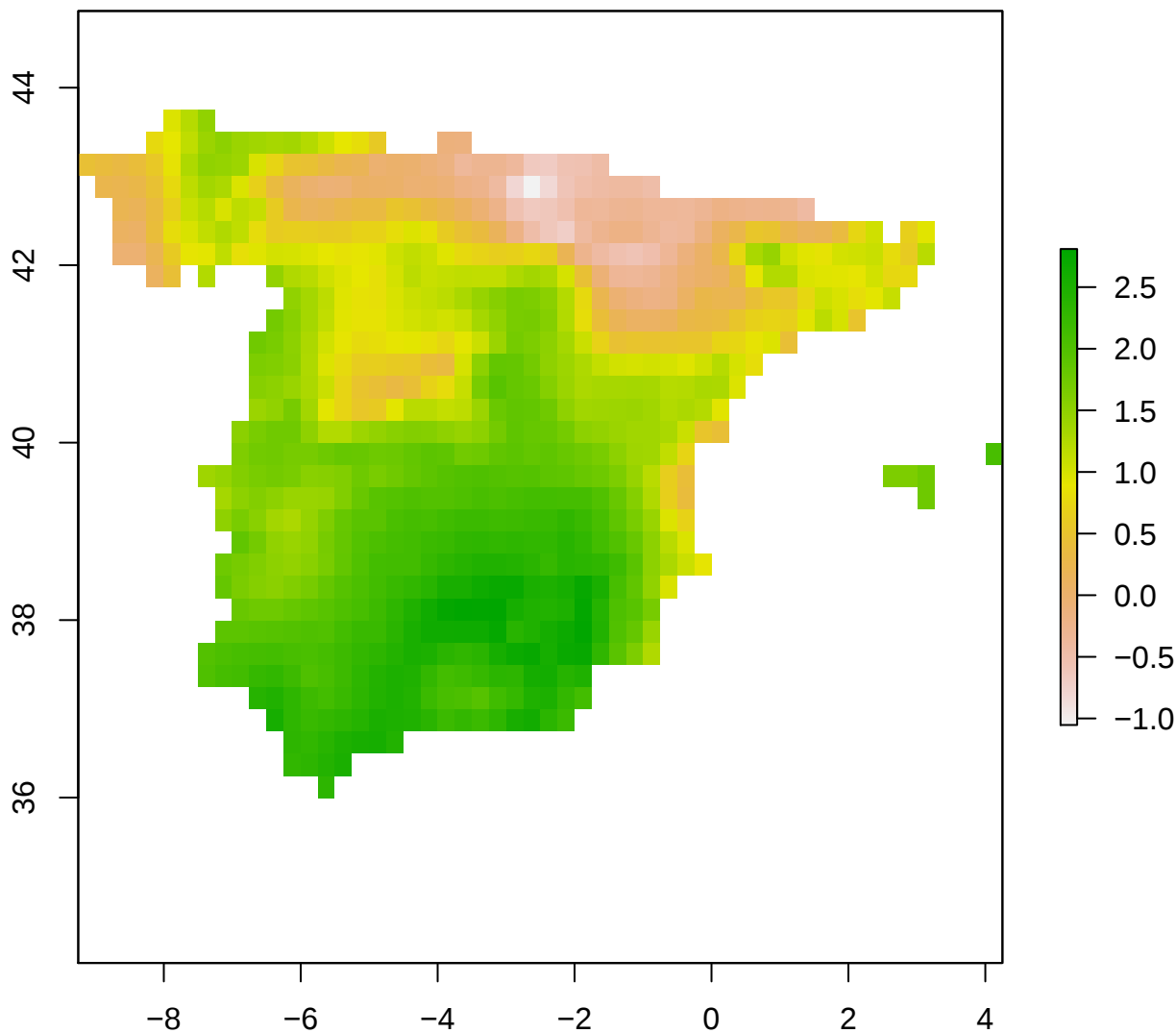
spi12_month - Spain 2010-11-01
