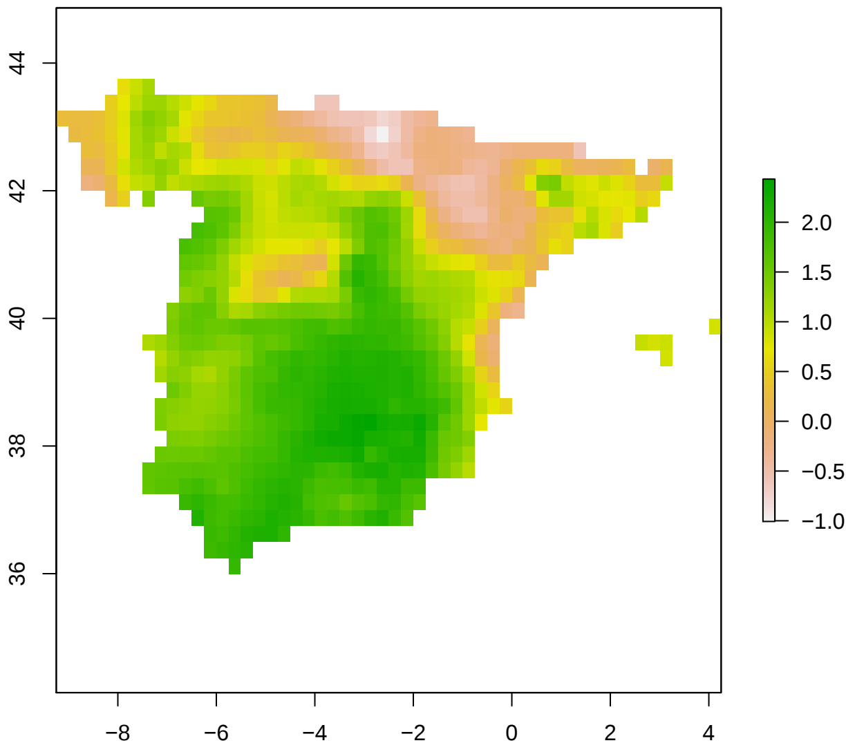
spi12_month - Spain 2010-09-01
