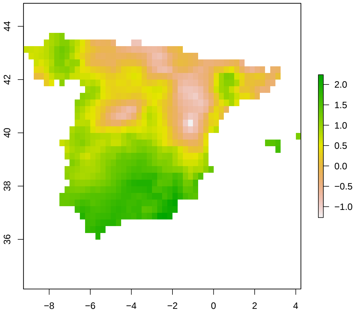
spi12_month - Spain 2010-03-01
