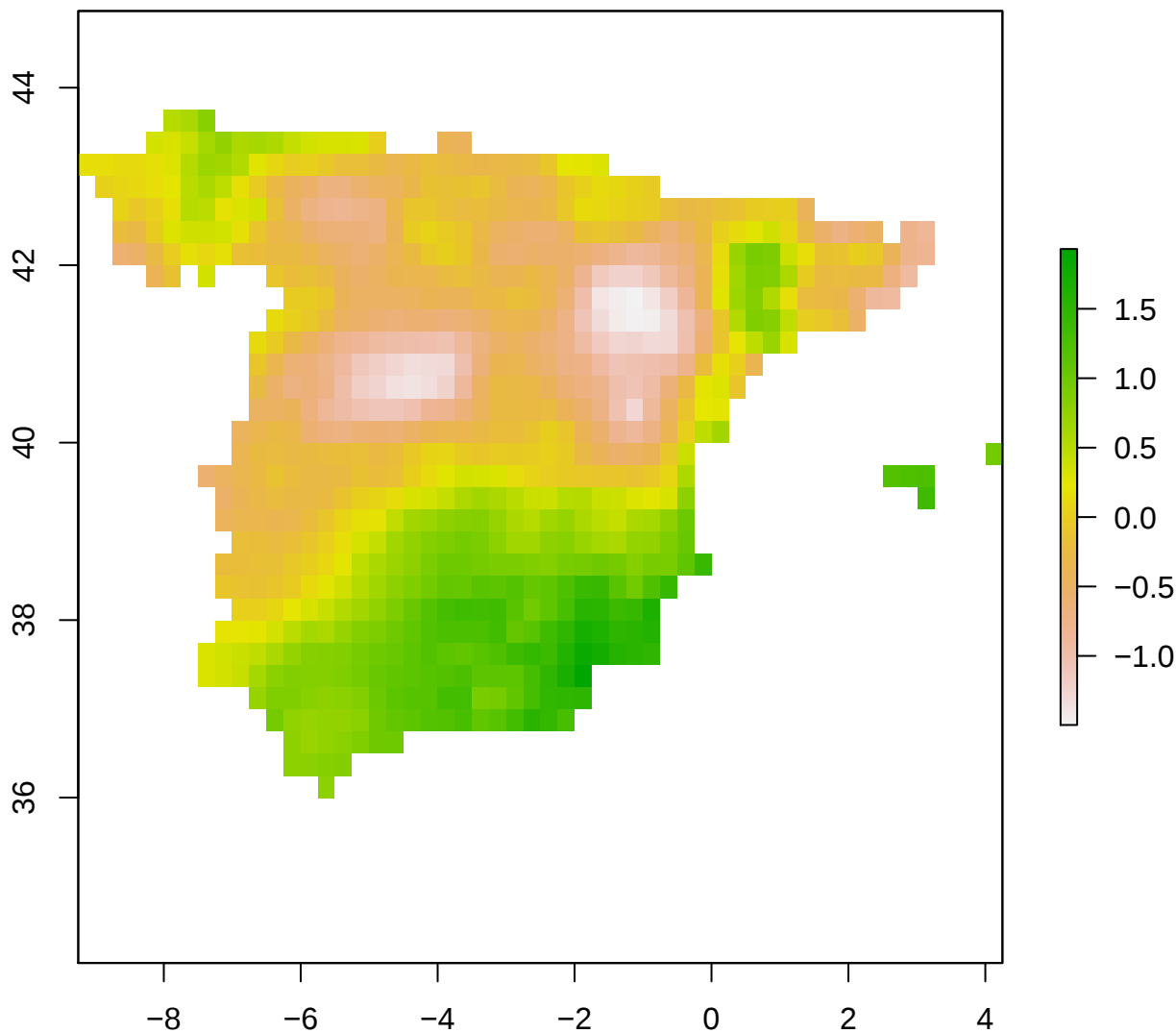
spi12_month - Spain 2010-01-01
