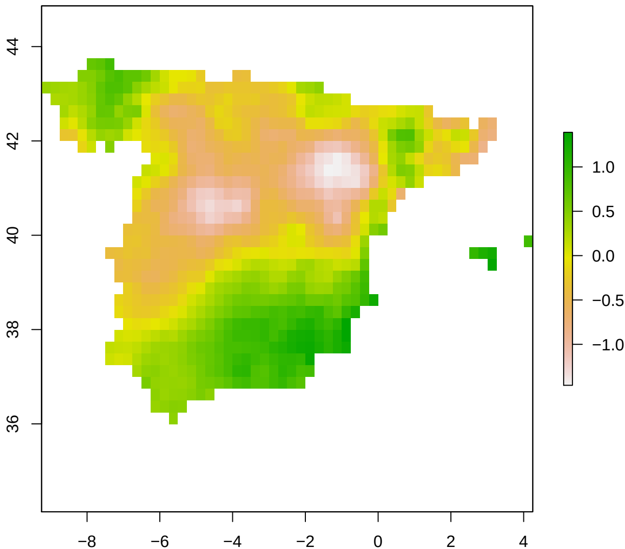
spi12_month - Spain 2009-12-01
