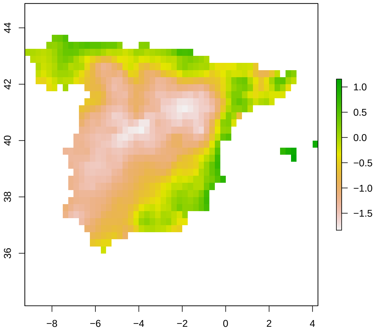
spi12_month - Spain 2009-11-01
