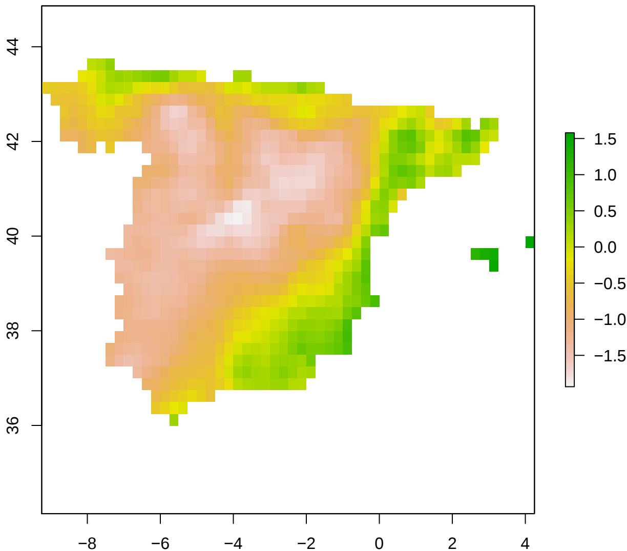
spi12_month - Spain 2009-10-01
