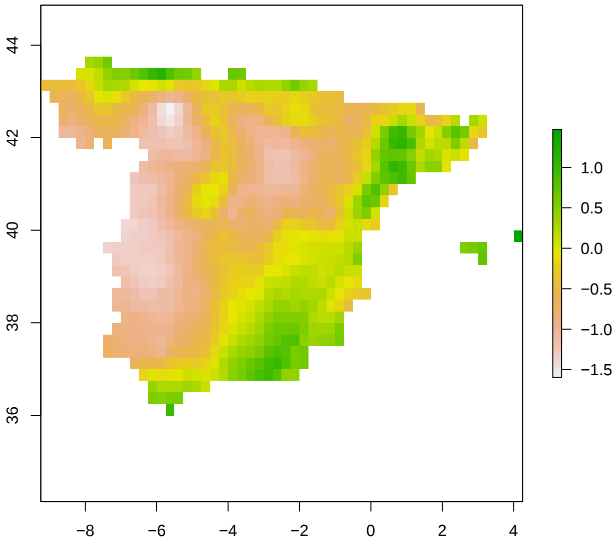
spi12_month - Spain 2009-08-01
