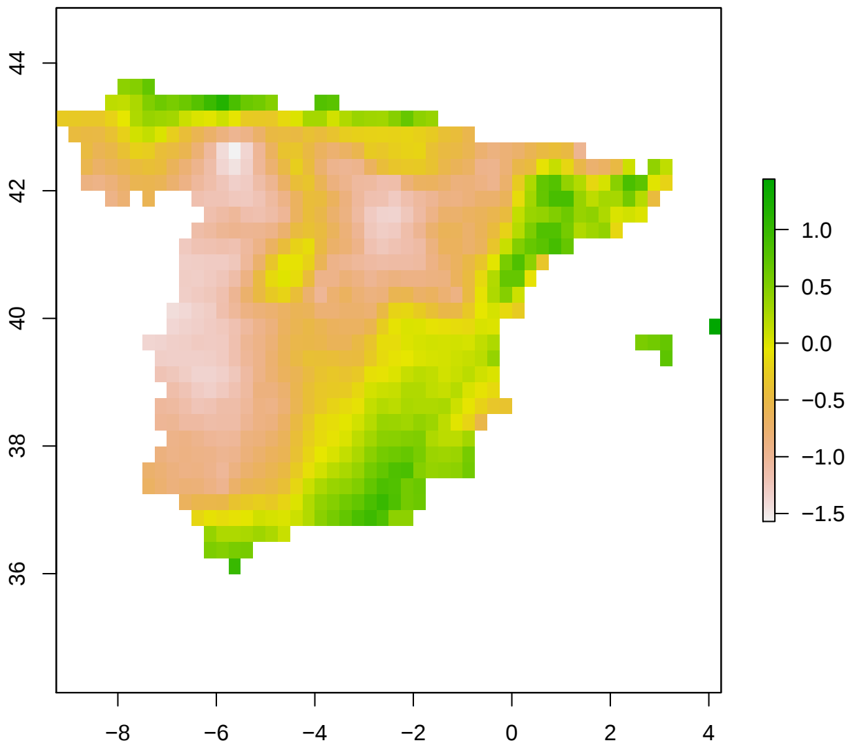
spi12_month - Spain 2009-07-01
