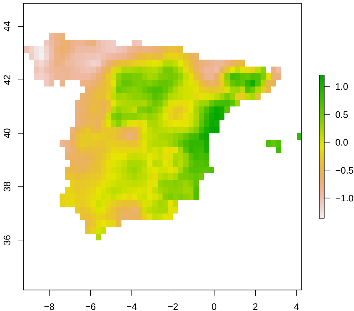
spi12_month - Spain 2008-09-01
