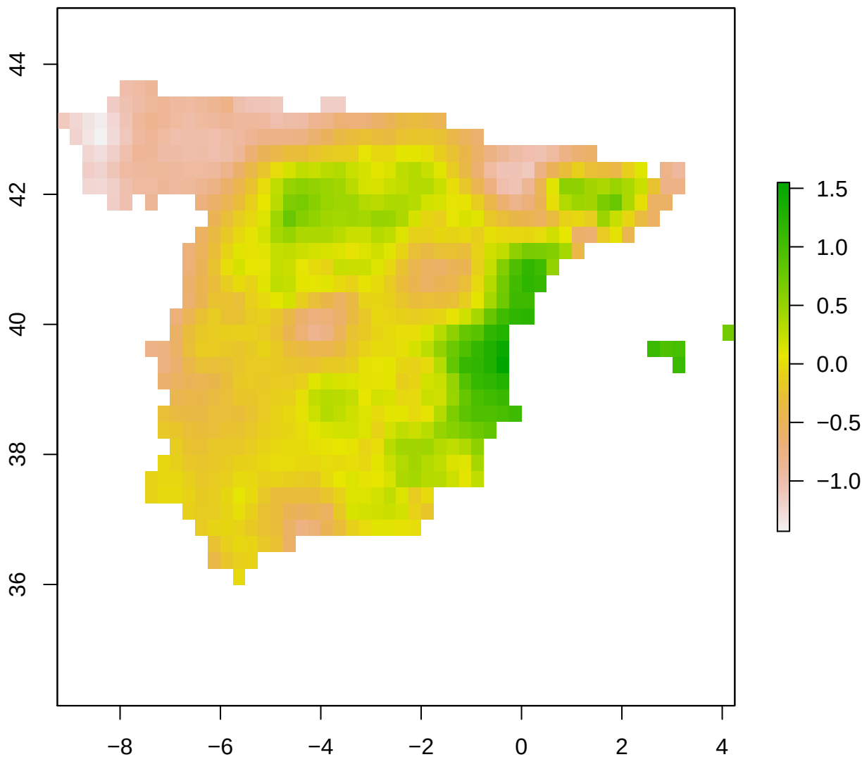
spi12_month - Spain 2008-08-01
