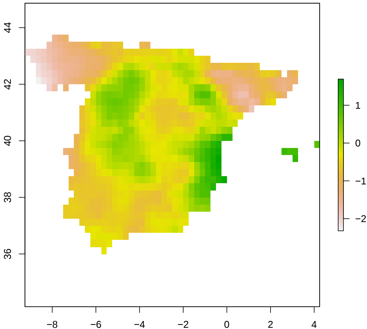
spi12_month - Spain 2007-12-01
