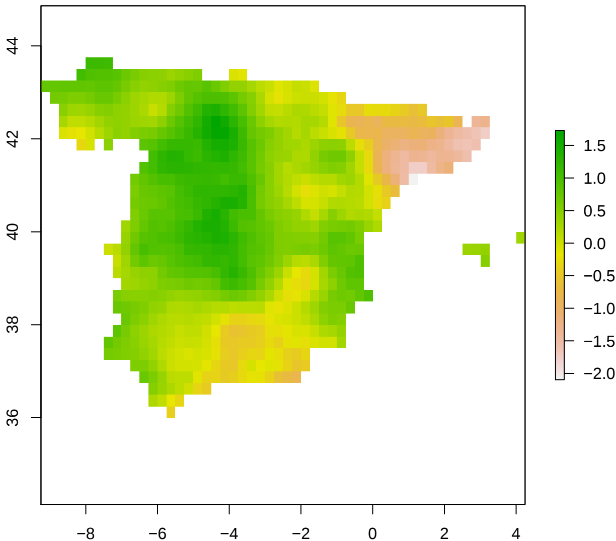
spi12_month - Spain 2007-09-01
