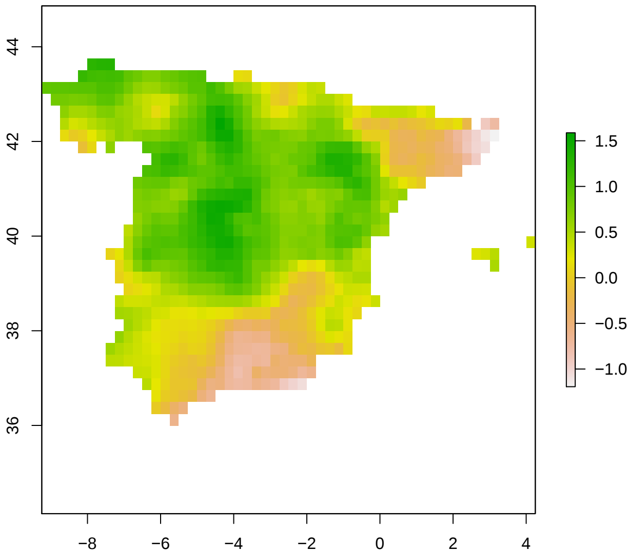
spi12_month - Spain 2007-08-01
