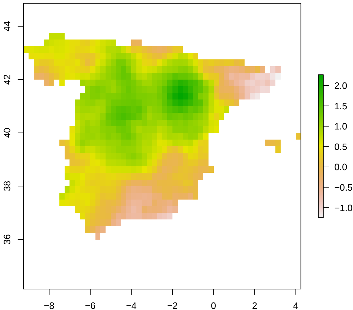
spi12_month - Spain 2007-05-01
