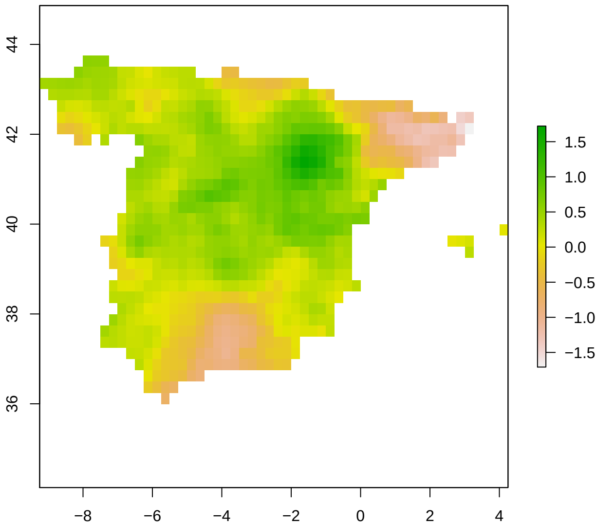
spi12_month - Spain 2007-04-01
