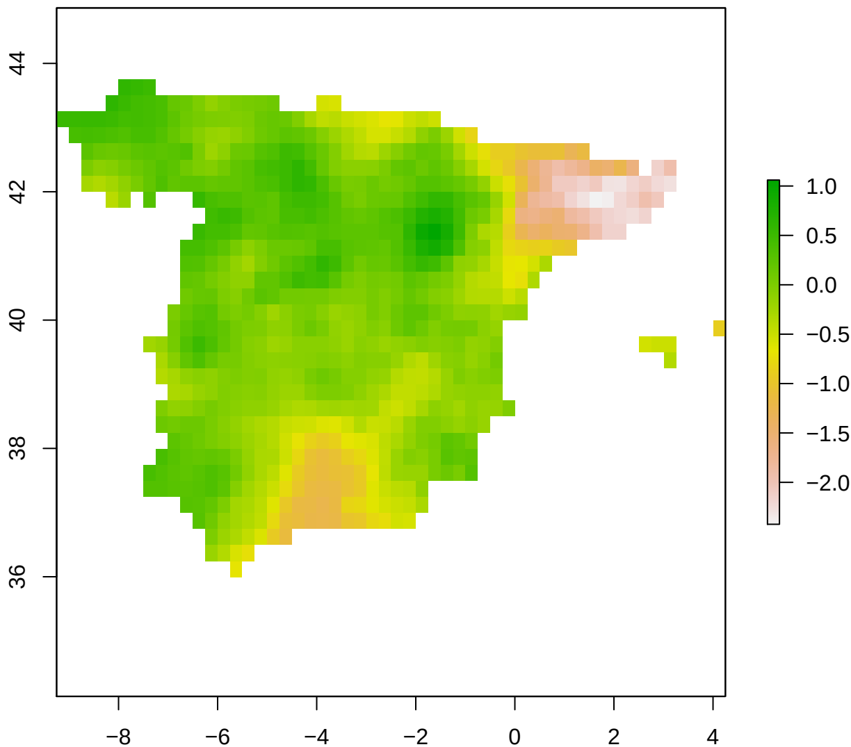
spi12_month - Spain 2007-03-01
