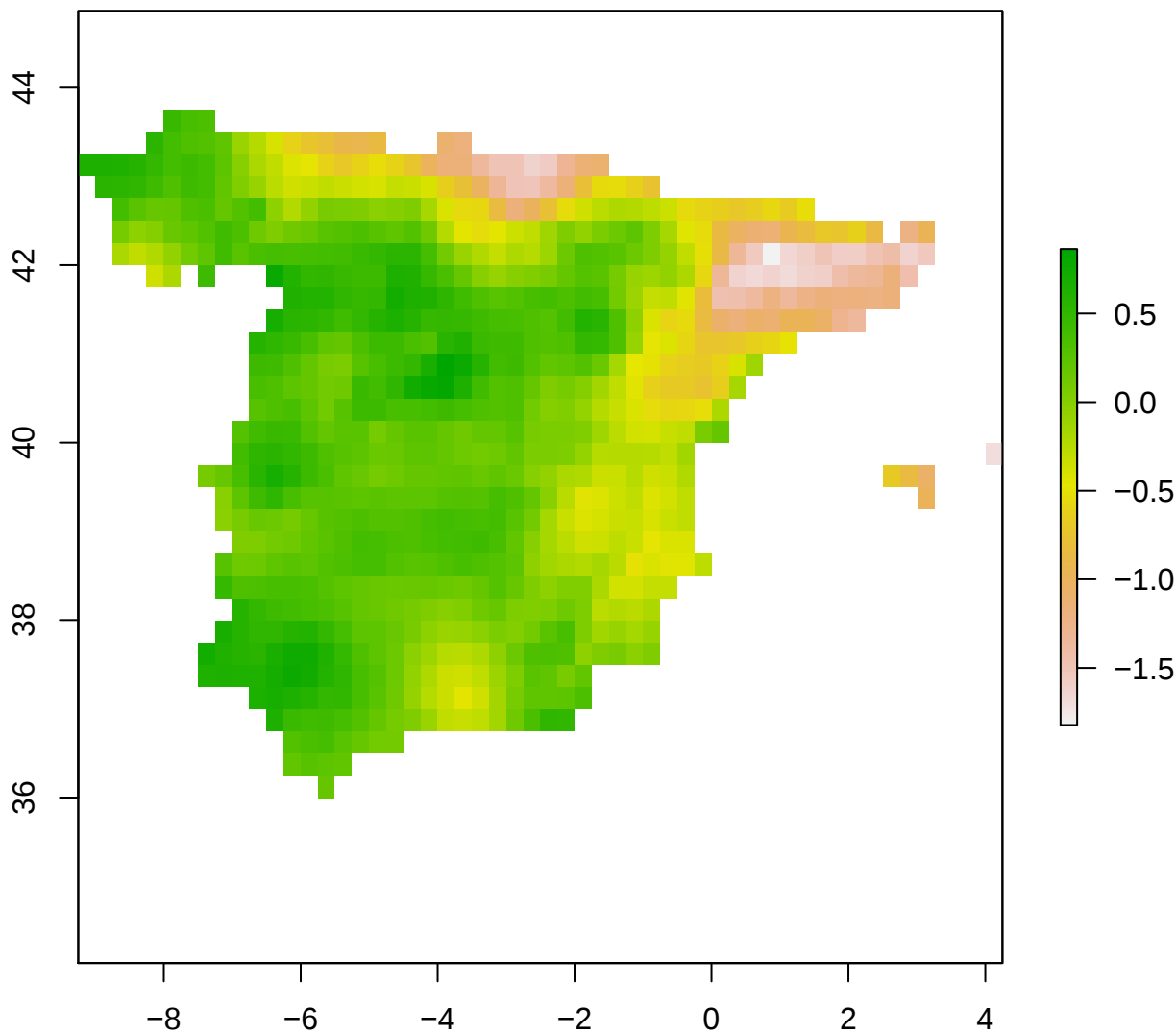
spi12_month - Spain 2006-11-01
