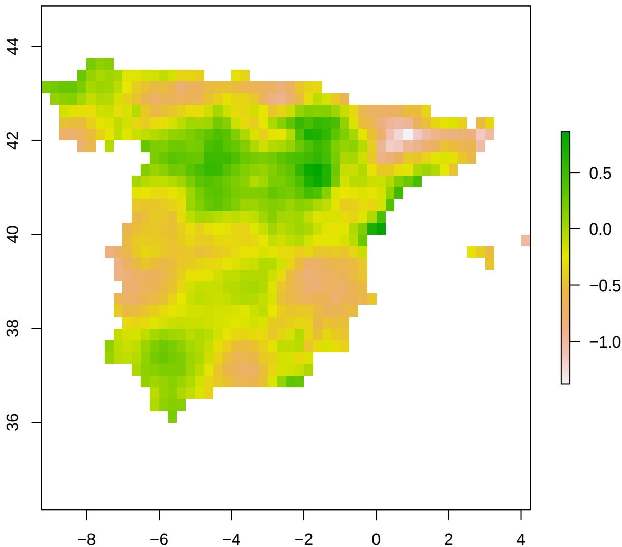
spi12_month - Spain 2006-10-01
