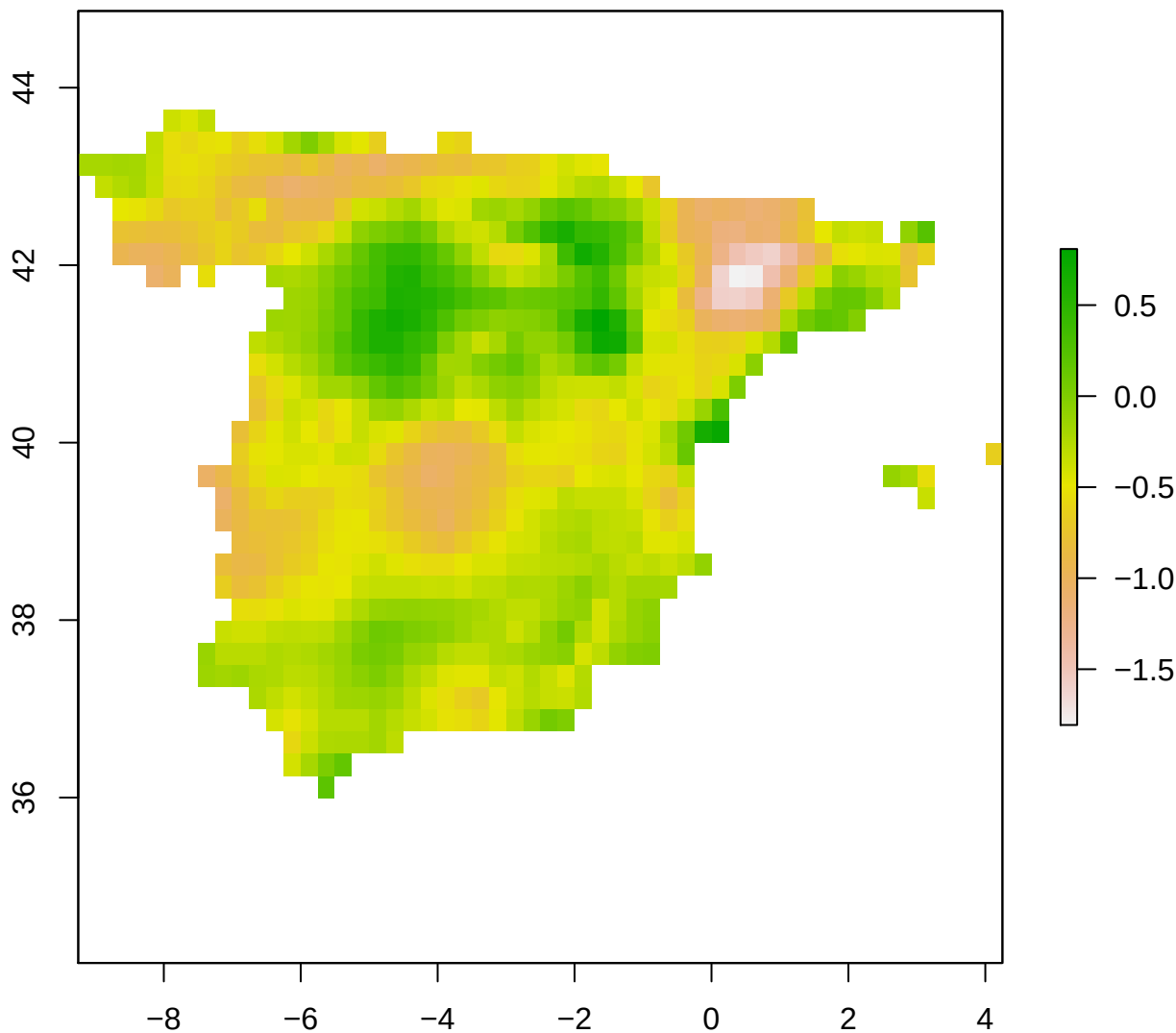
spi12_month - Spain 2006-08-01
