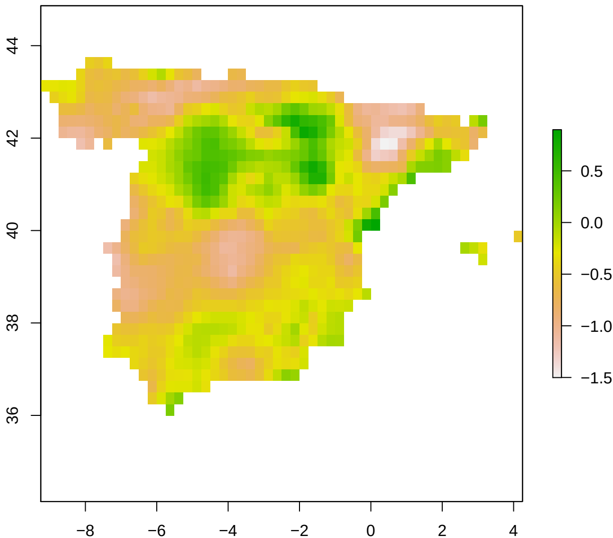
spi12_month - Spain 2006-07-01
