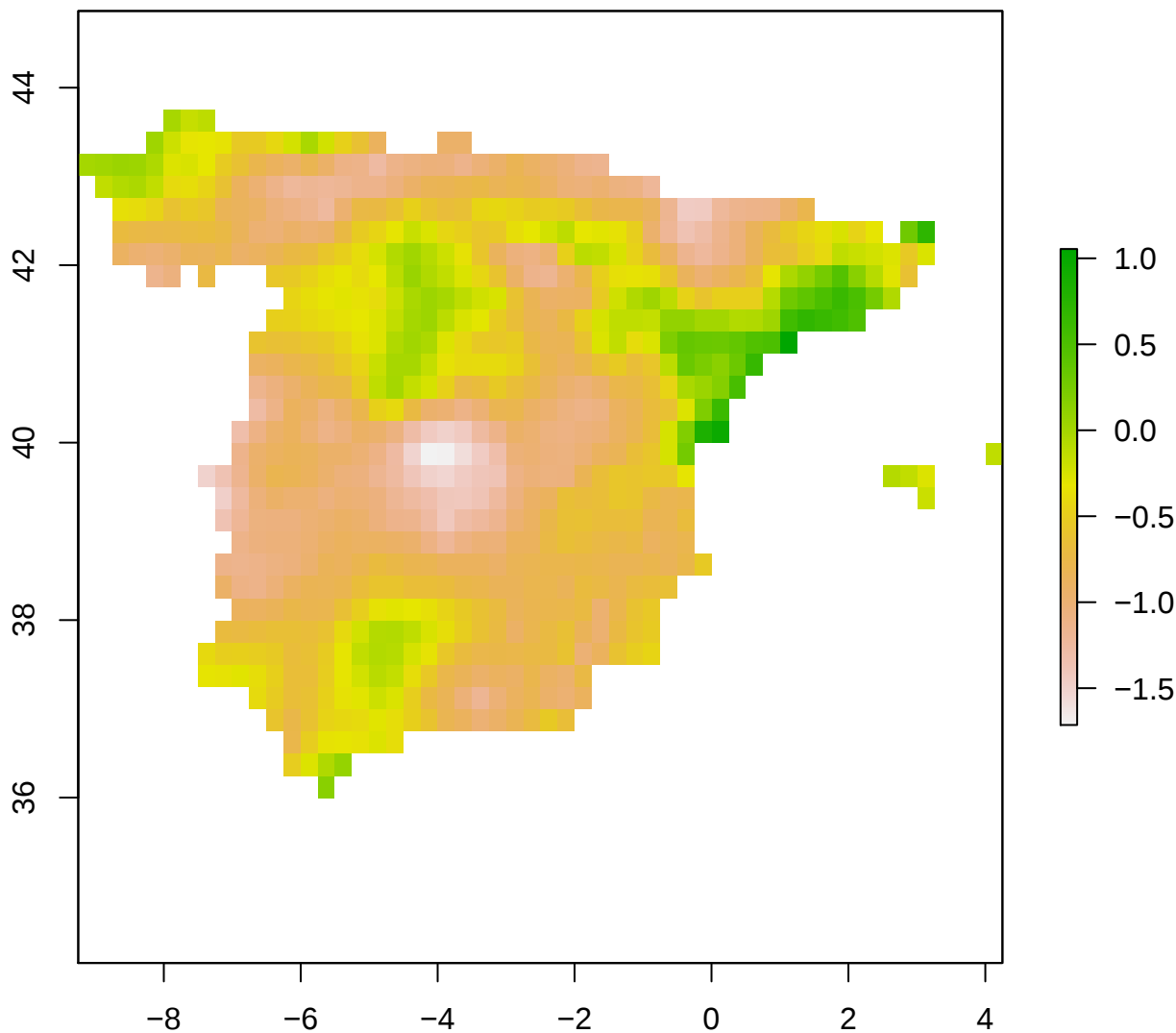
spi12_month - Spain 2006-04-01
