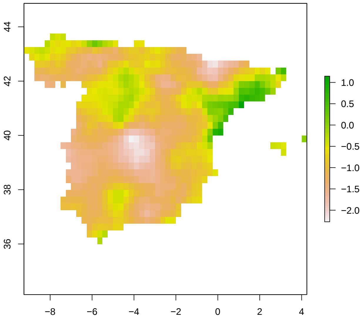
spi12_month - Spain 2006-02-01
