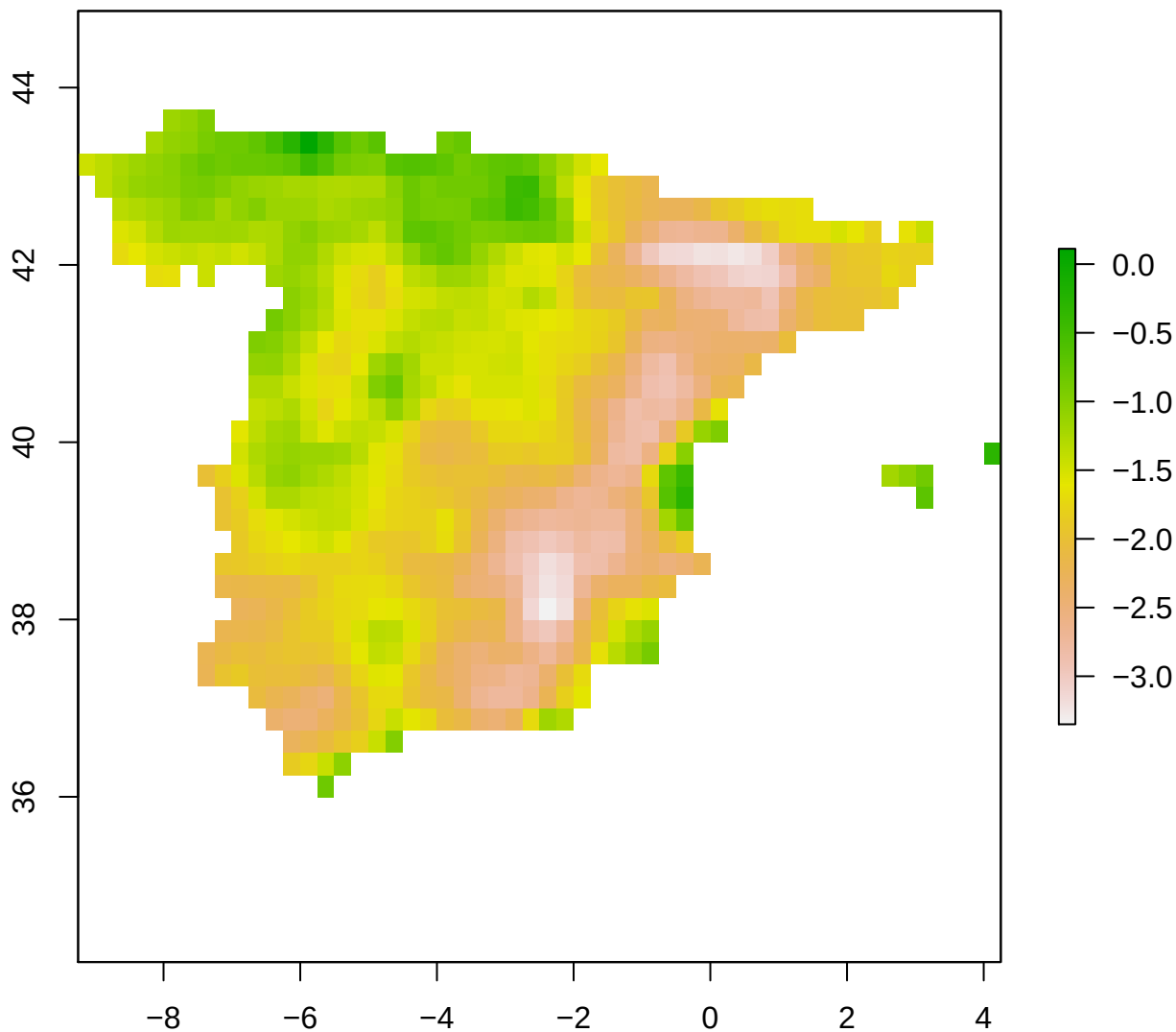
spi12_month - Spain 2005-05-01
