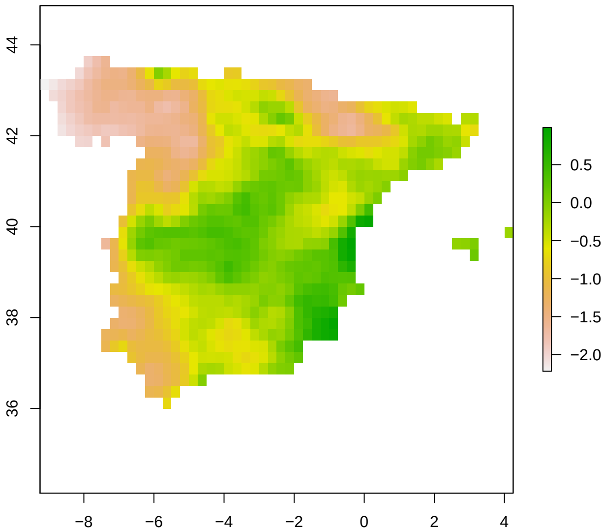
spi12_month - Spain 2005-01-01
