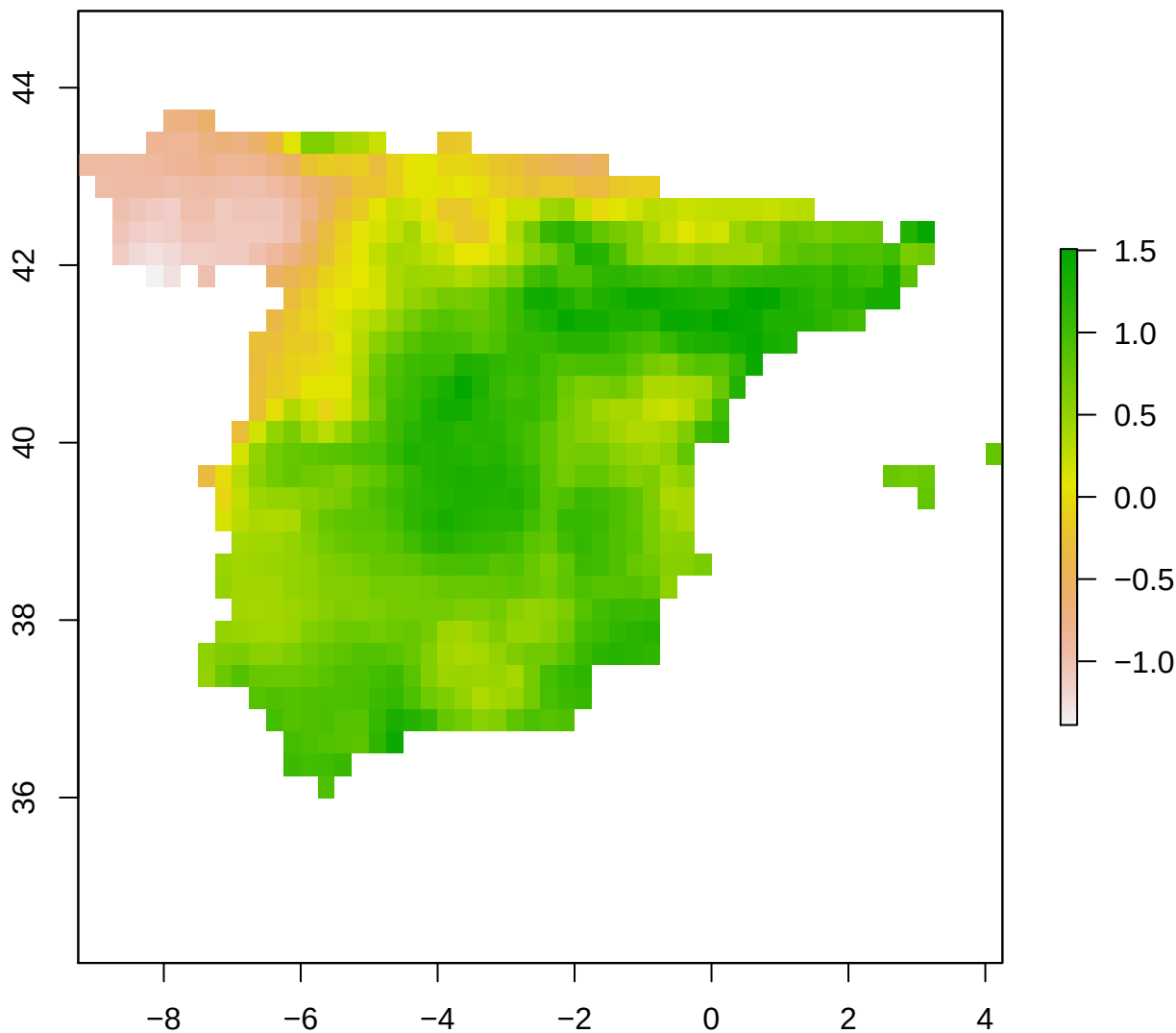
spi12_month - Spain 2004-07-01
