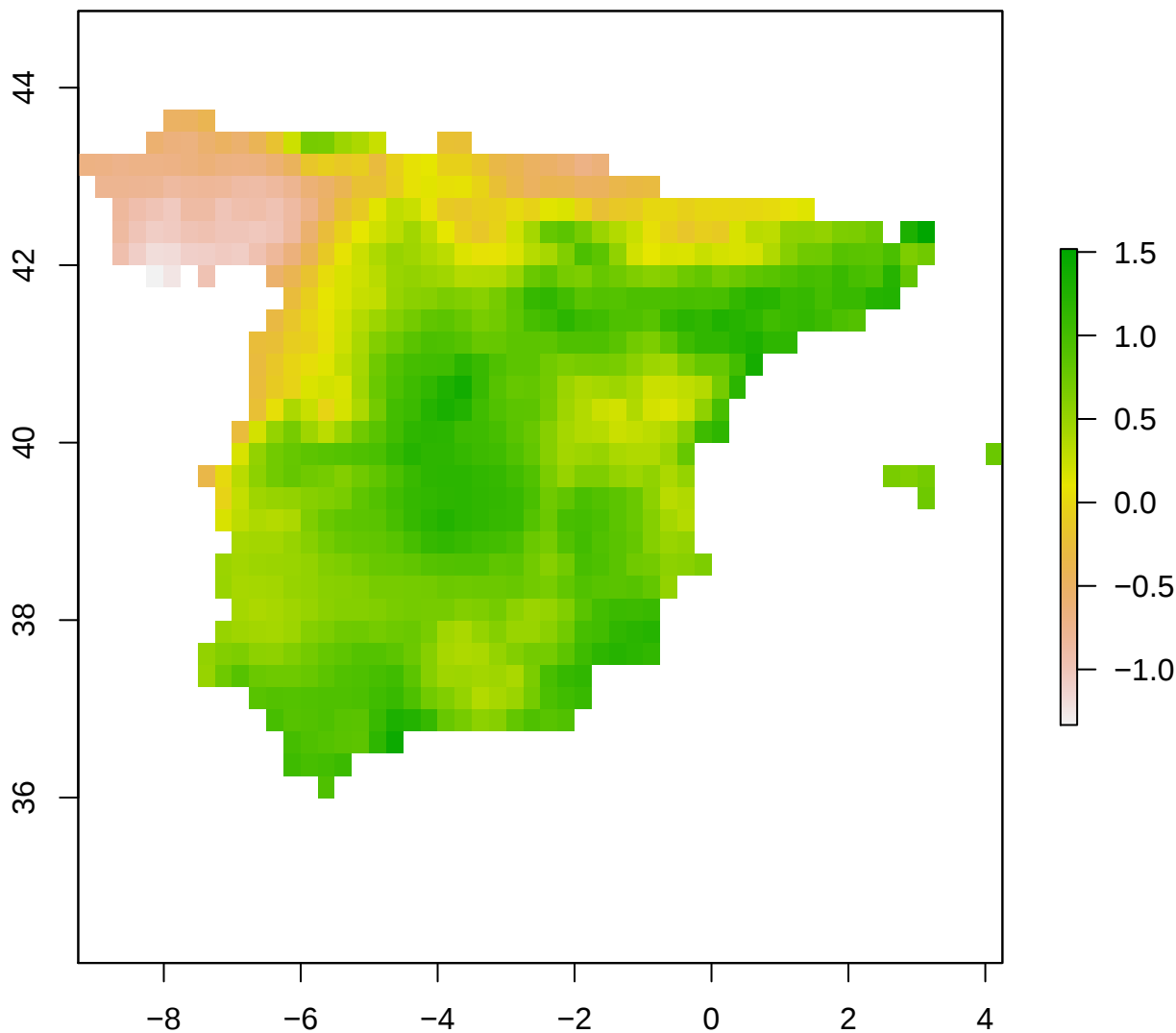
spi12_month - Spain 2004-06-01
