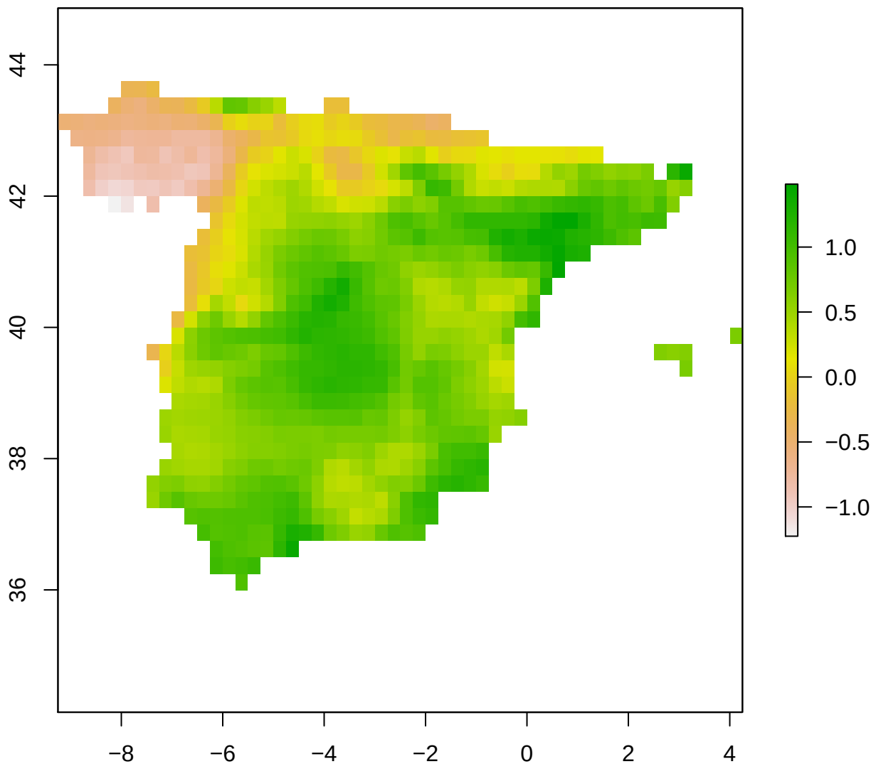
spi12_month - Spain 2004-05-01
