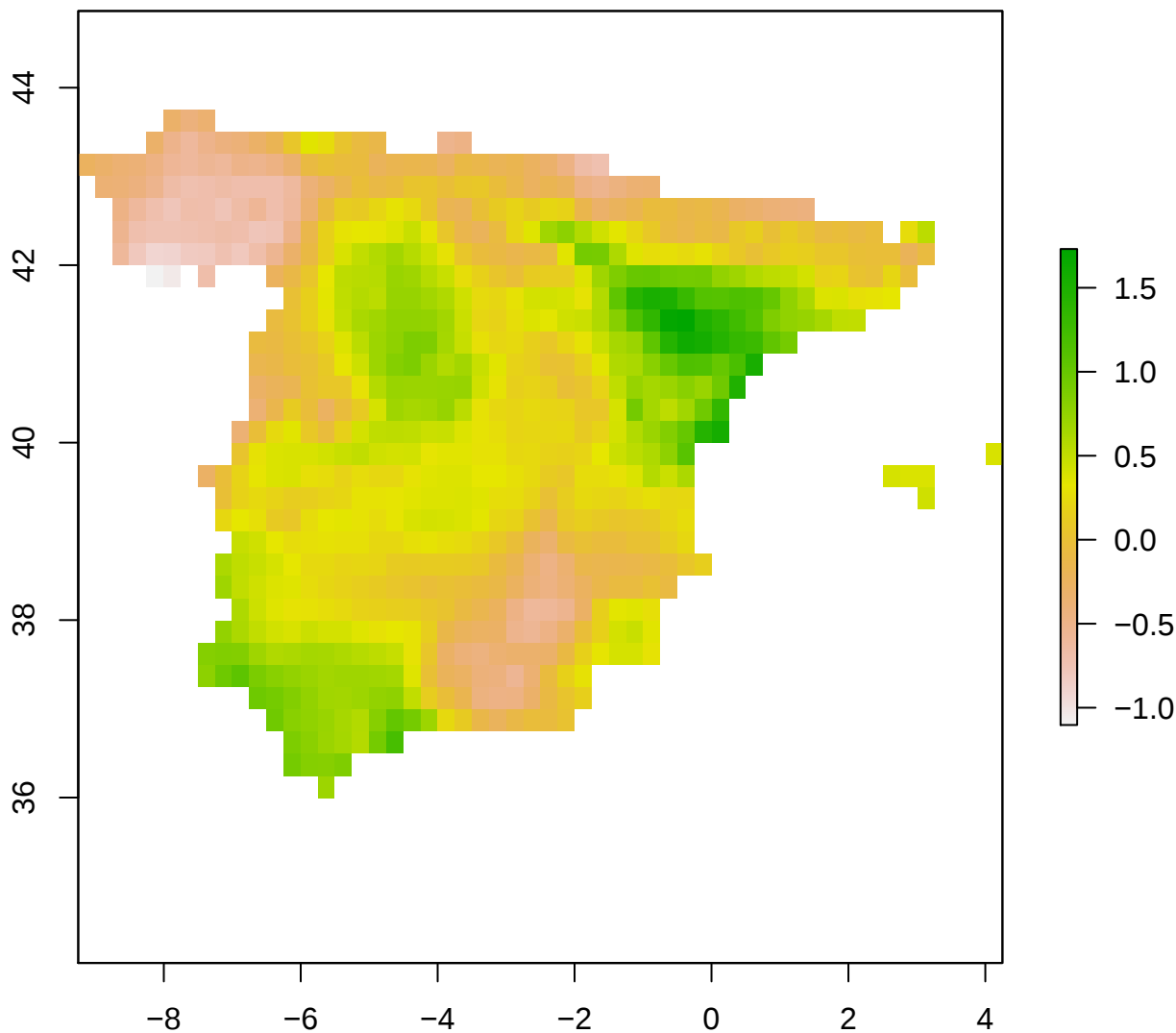
spi12_month - Spain 2004-03-01
