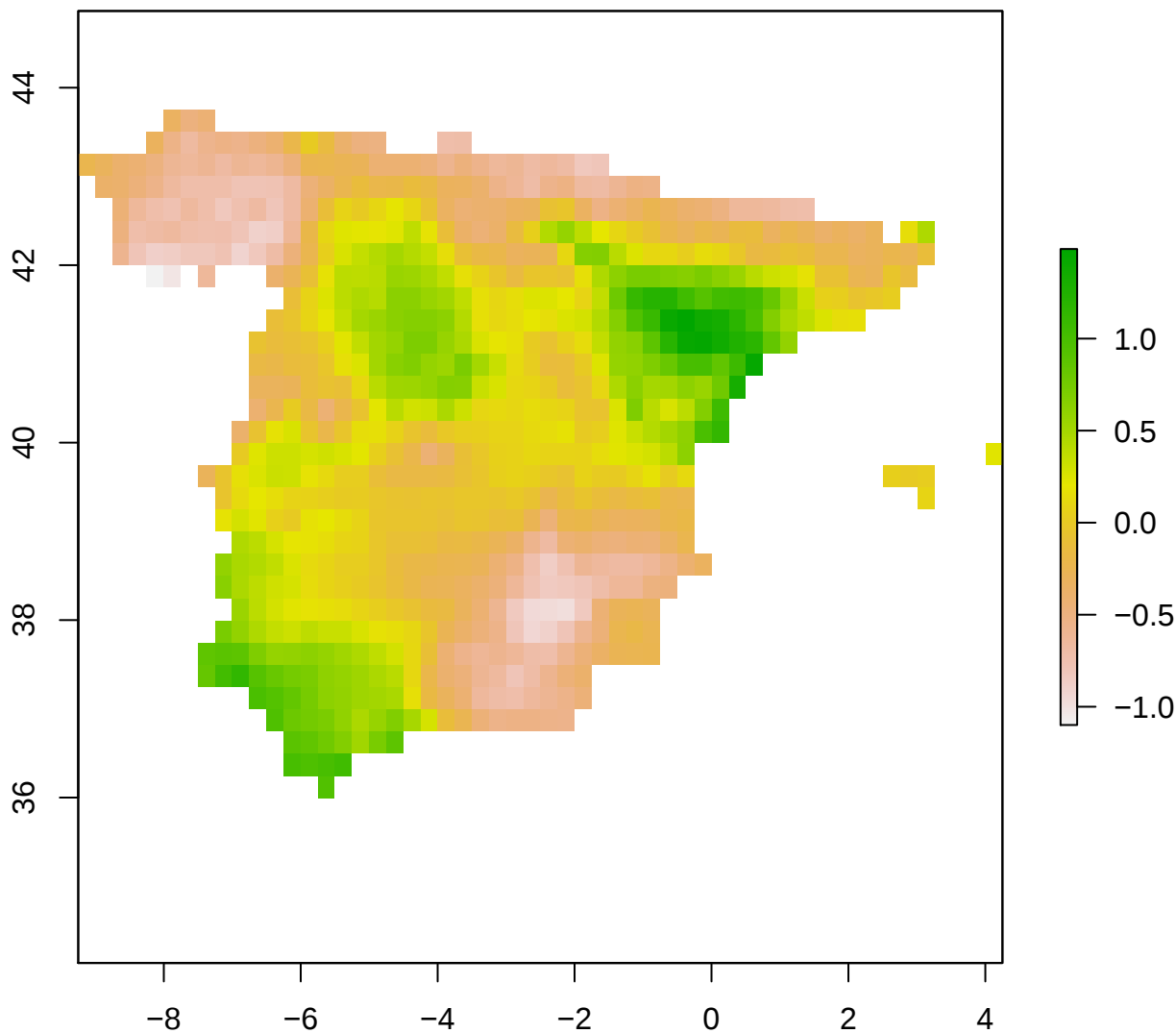
spi12_month - Spain 2004-02-01
