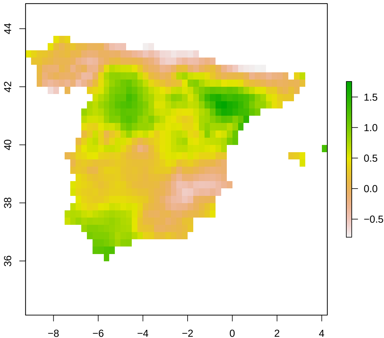
spi12_month - Spain 2003-12-01
