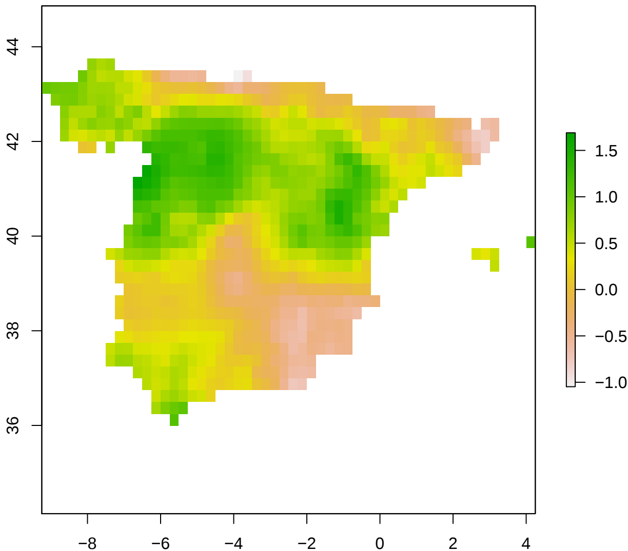
spi12_month - Spain 2003-07-01
