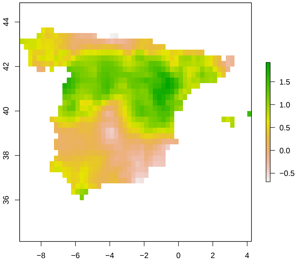
spi12_month - Spain 2003-05-01
