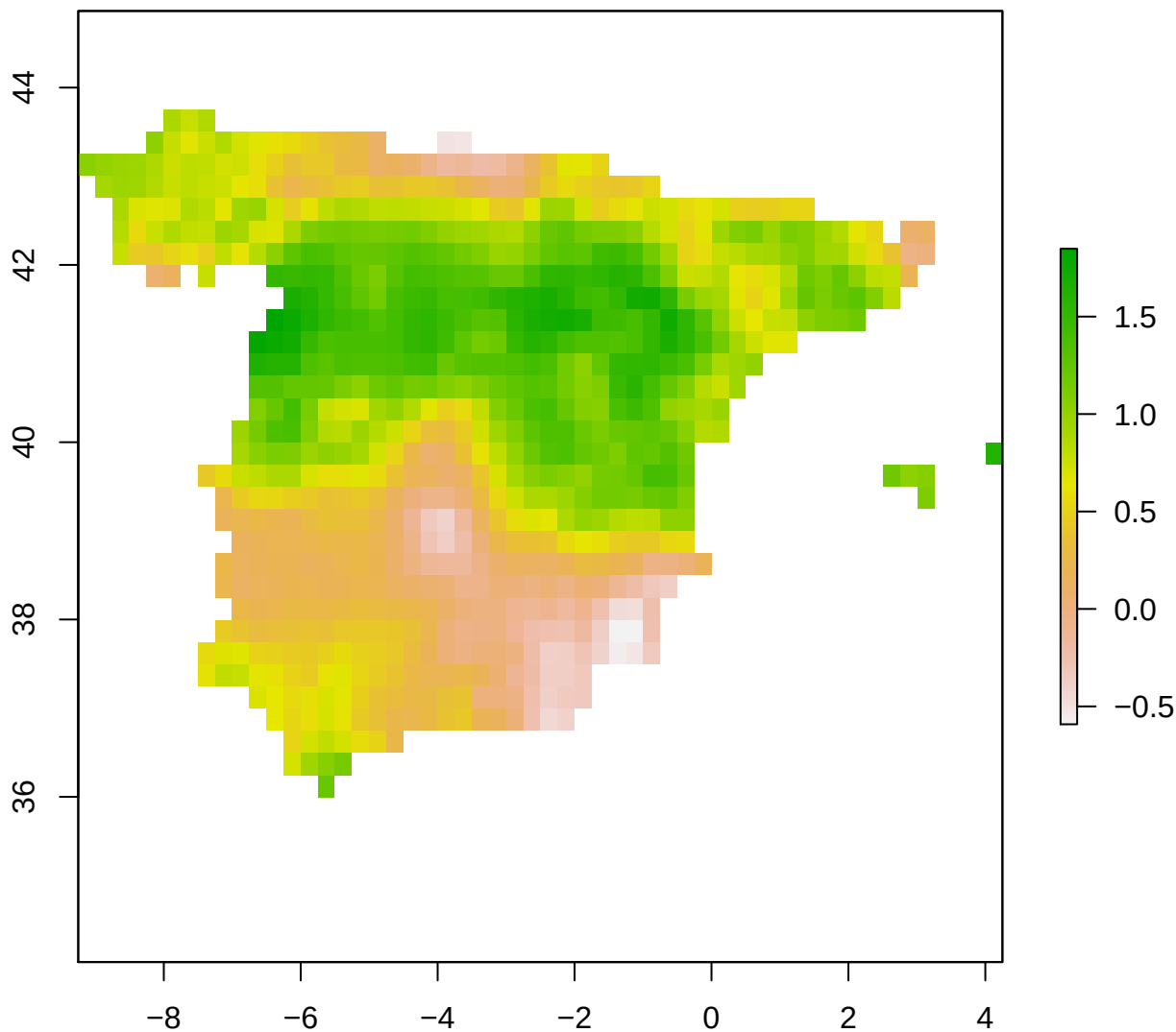
spi12_month - Spain 2003-04-01
