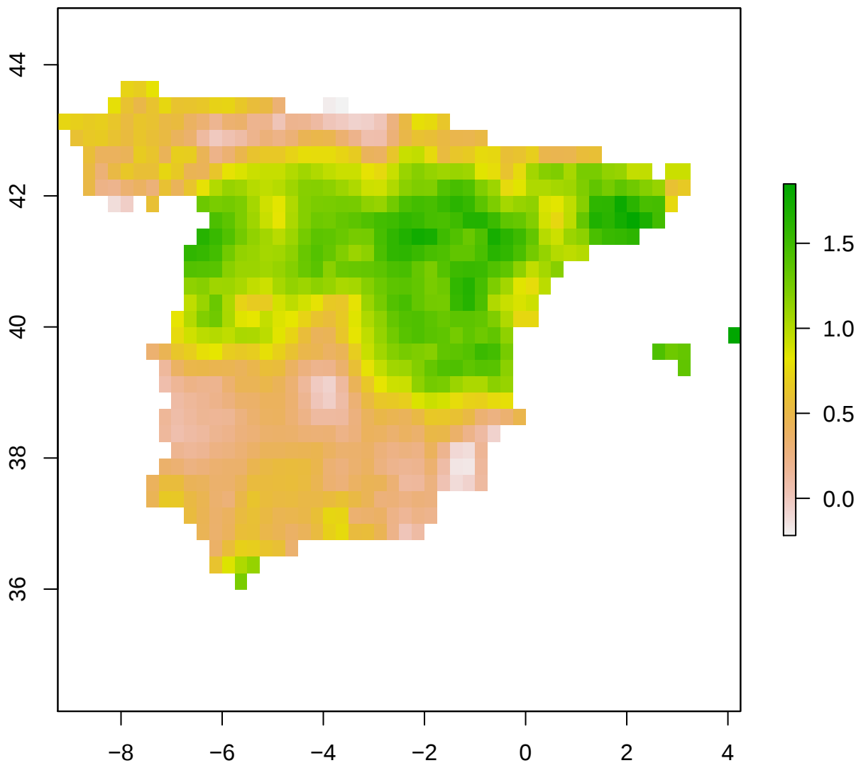
spi12_month - Spain 2003-03-01
