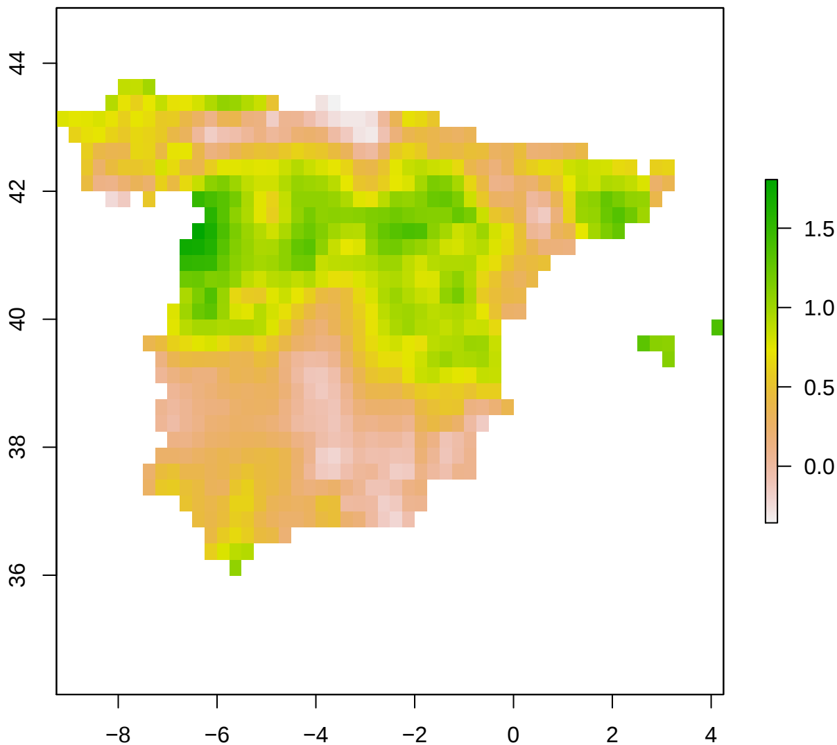
spi12_month - Spain 2003-01-01
