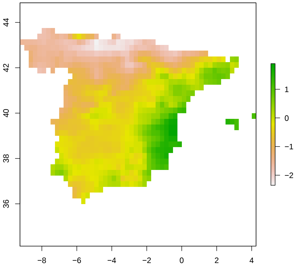
spi12_month - Spain 2002-08-01
