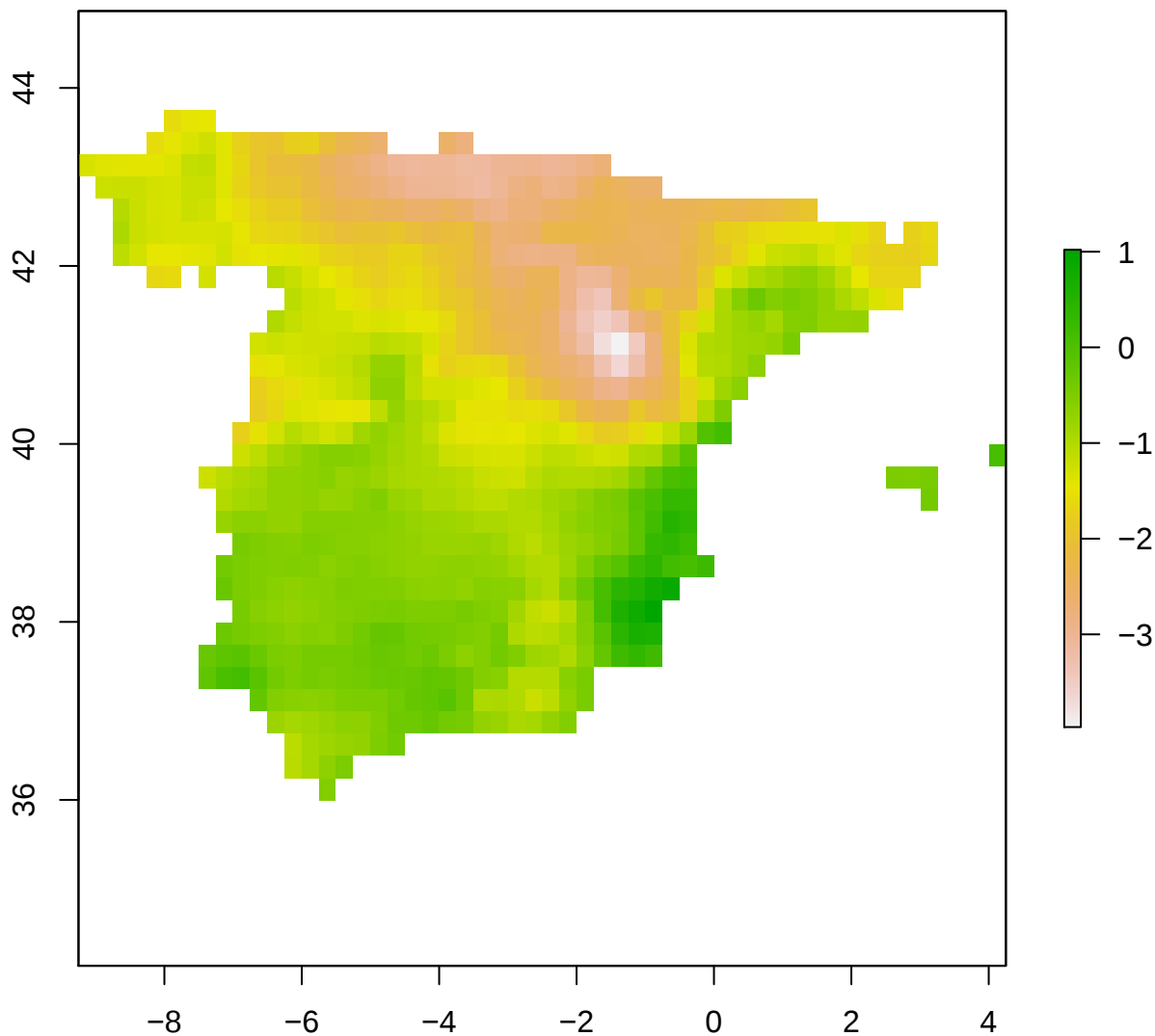
spi12_month - Spain 2002-03-01
