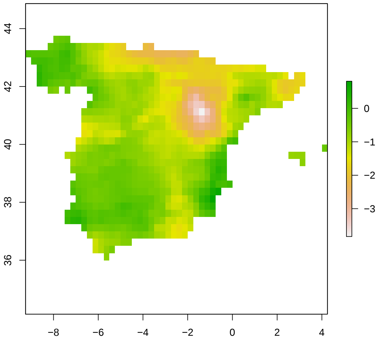
spi12_month - Spain 2002-02-01
