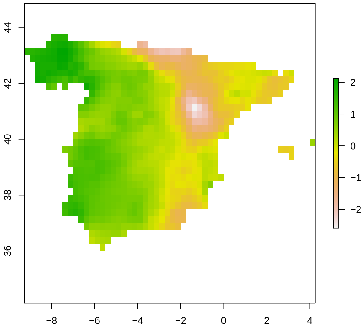
spi12_month - Spain 2001-11-01
