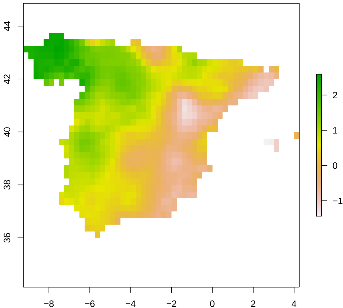
spi12_month - Spain 2001-05-01
