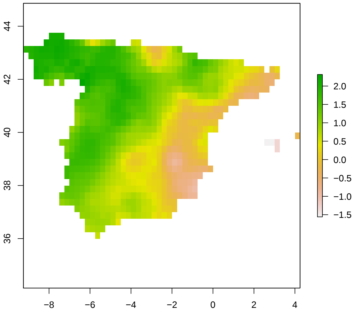
spi12_month - Spain 2001-02-01
