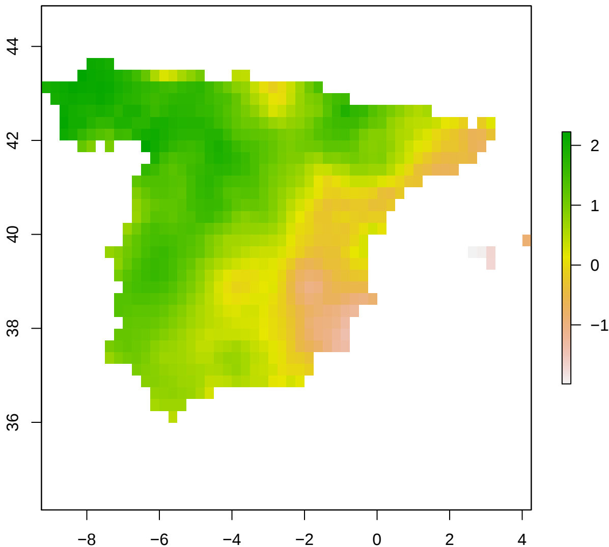
spi12_month - Spain 2001-01-01
