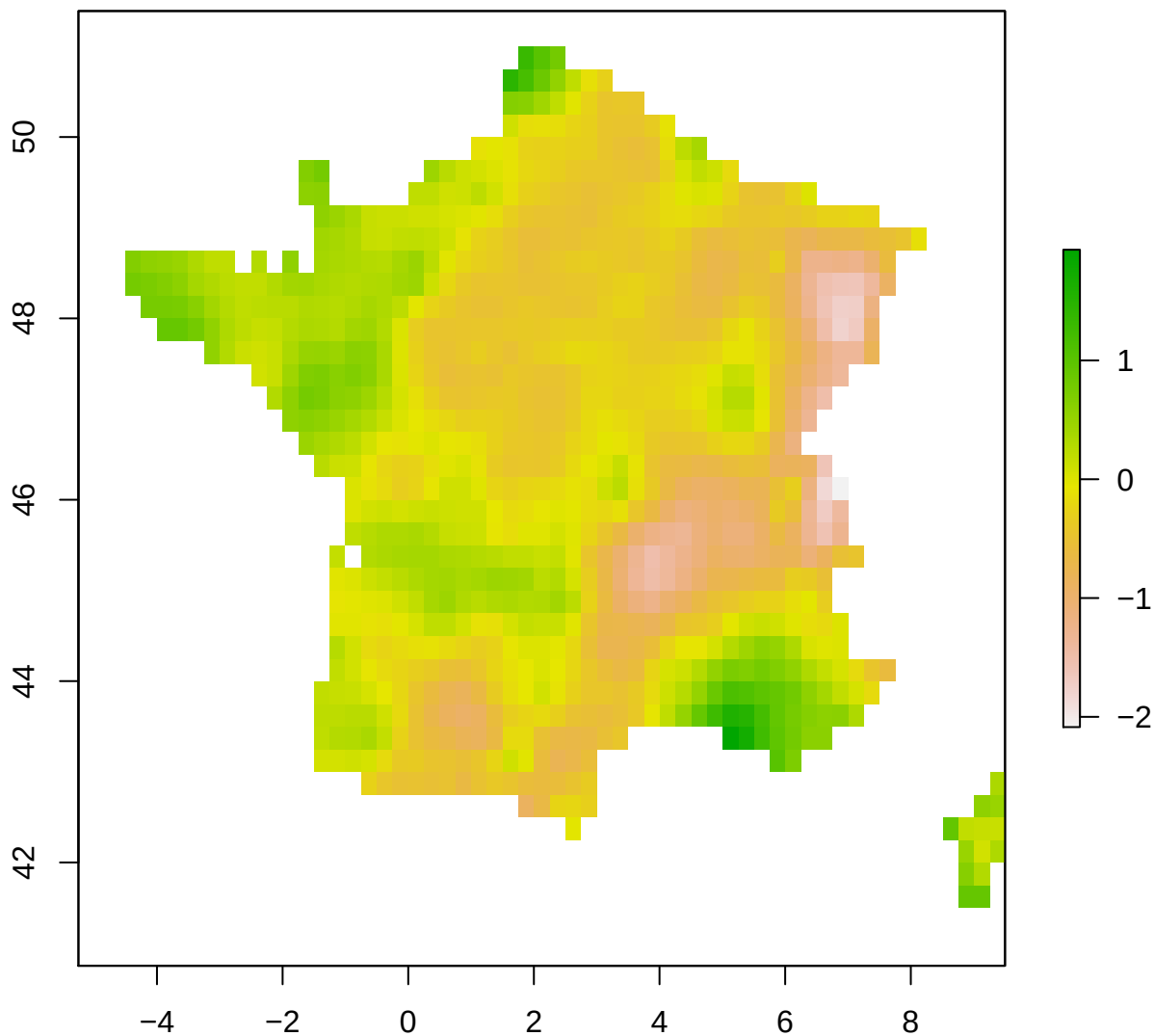
spi12_month – France 2010-03-01
