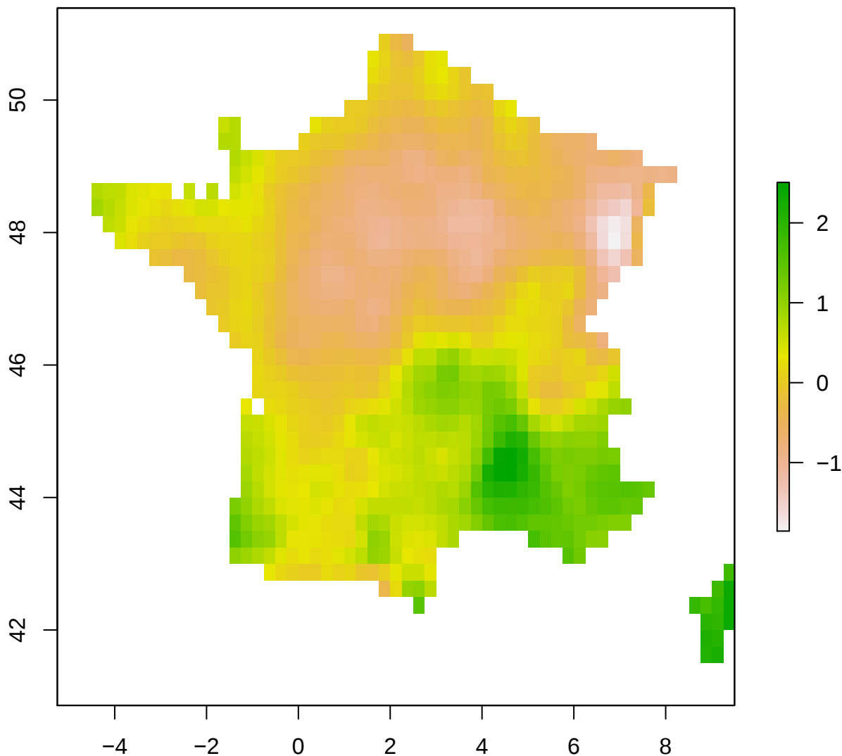
spi12_month – France 2009-04-01
