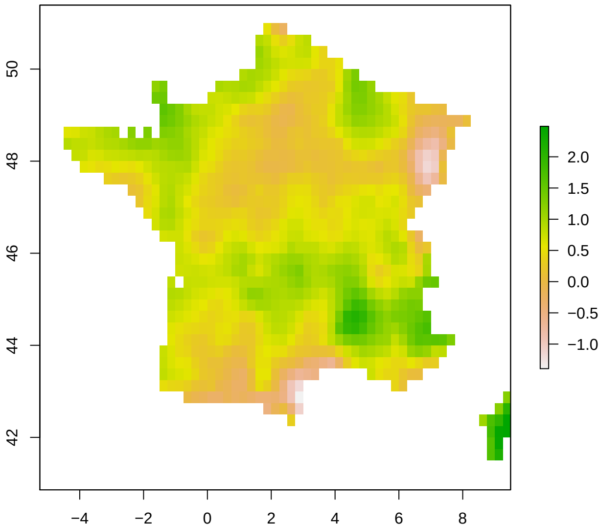
spi12_month – France 2008-11-01
