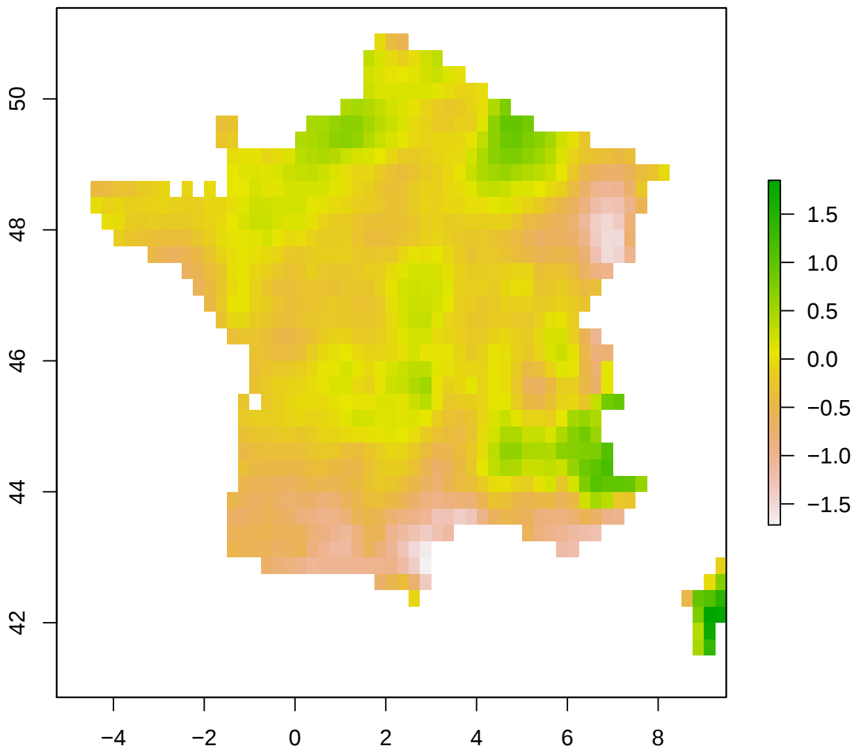
spi12_month – France 2008-08-01
