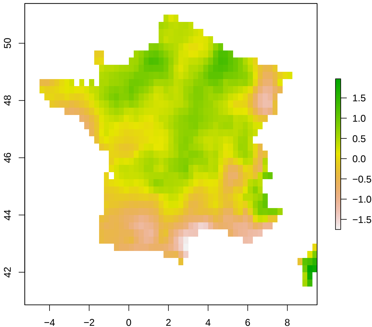
spi12_month – France 2008-06-01
