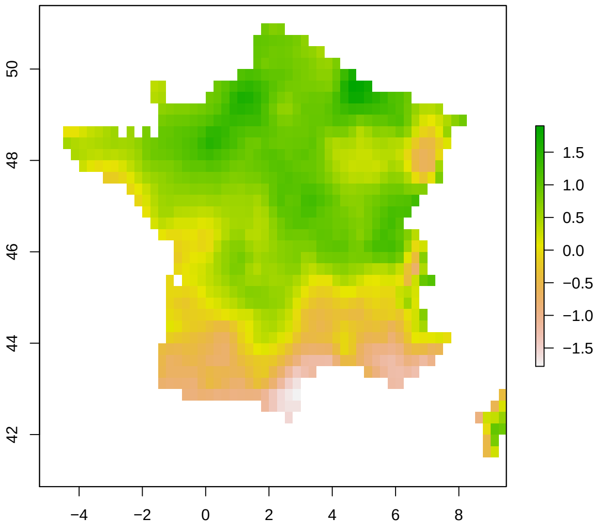
spi12_month – France 2008-04-01
